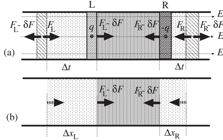
Figure 4: (a) A gas contained in a cylinder is compressed under the action of two pistons, L, with electric charge +q fixed to it, and R, with electric charge -q fixed to it. On piston L, a force F_L = qE is exerted by the electric field E and a force -(F_L - \delta F) slightly smaller by the gas. On piston R a force F_R = -qE is exerted by the electric field, and a force (F_R - \delta F) by the gas. (b) Thus the gas is compressed under the action of force F_L applied to a displacement \Delta x_L and a force F_R applied to a displacement \Delta x_R . Both forces F_L and F_R are applied simultaneously during time interval \Delta t . Every piston acts as an intermediate agent between the work reservoir (electric field and battery to which the capacitor is connected) and the thermodynamics system (the gas).
