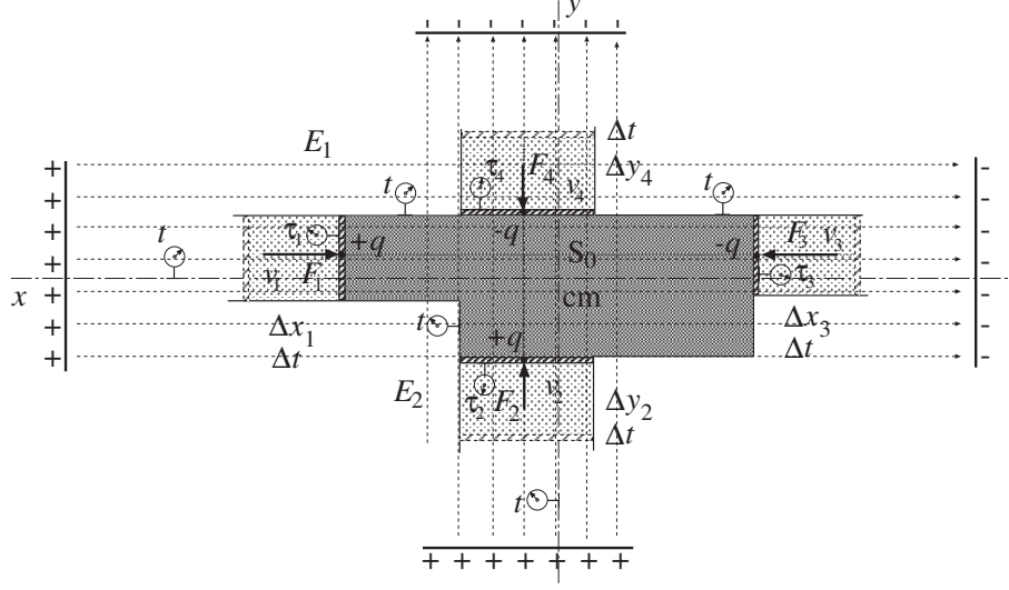
Figure 3: Extended system, with k pistons ( k = 1, 2, 3, 4 ), to which forces F_k = qE_k are simultaneously applied during time interval \Delta t as measured in frame S_0 by a set of synchronized clocks at rest (Fig. 1). On the k -th piston there is a clock that measures its proper time \tau_k . The k -th piston displaces d\mathbf{r}_k during time interval dt , speed \mathbf{v}_k = d\mathbf{r}_k/dt and proper time interval d\tau_k . Forces F_k have an electromagnetic origin: an electric field E_k , produced by a plane-parallel charged capacitor, interacts with a charge q_k fixed to the k -th piston.
