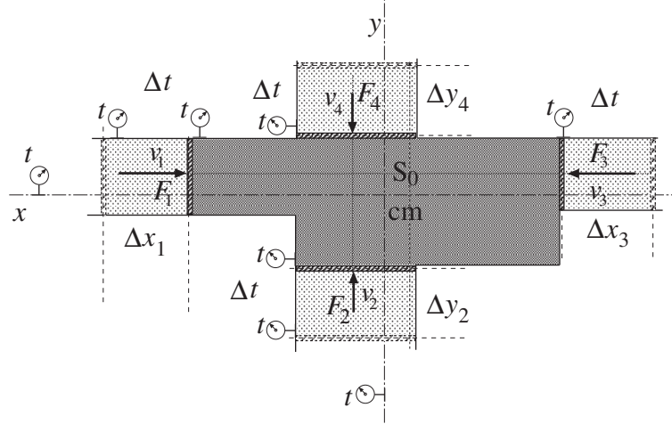
Figure 2: Compression process in frame S_0 . A set of external forces F_k ( k = 1, 2, 3, 4 ) are applied on an extended, deformable system during the same time interval \Delta t , as measured in frame S_0 , with zero total impulse and zero torque. The k -th force has associated the displacement \Delta \mathbf{r}_k ( \mathbf{r} = (x, y) ) and 3-vector velocity \mathbf{v}_k = \Delta \mathbf{r}_k / \Delta t . The center-of-mass (cm) of the system does not move during the process.
