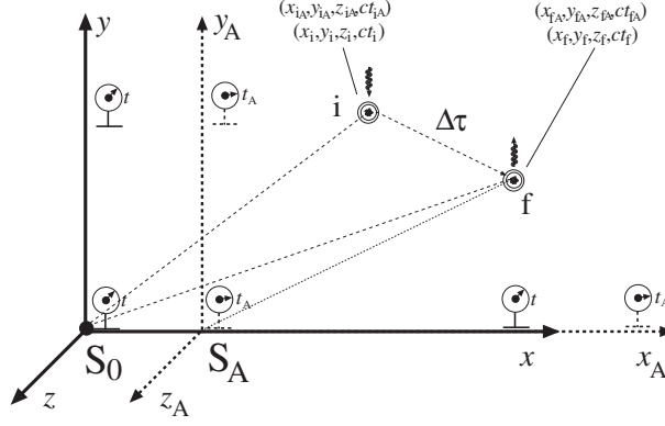
Figure 9: Frames S_0 and S_A in ‘standard configuration’. Axes y and z in both frames are parallel and frame S_A moves with velocity V along axis x of frame S_0 . At time t = t_A = 0 origins coincide. Every frame has its own set of synchronized clocks. (i) Initial event, atom photon absorption, (f) final event, atom photon emission. \Delta\tau is the proper time of the atom (measured by a clock that travels with it) between events i and f.
