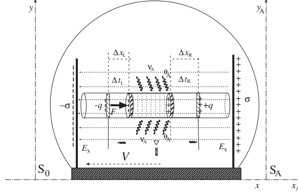
Figure 8: Isothermal compression given in Fig. 7, described from the point of view of an observer in frame S_A , standard configuration, with velocity V with respect to frame S_0 . In frame S_A forces are not applied simultaneously and heat carries linear momentum.
