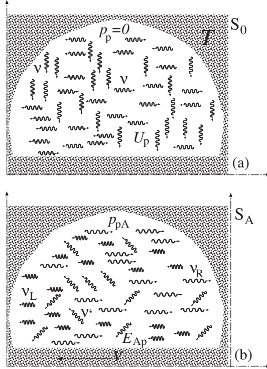
Figure 5: (a) Cavity with walls at temperature T filled with thermal radiation (photons) frequency \nu = \nu(T) (monochromatic approximation). In frame S_0 linear momentum for this ensemble of photons is zero p_p = 0 and its energy function is U_p = Nh\nu . (b) In frame S_A , the same ensemble of photons, with frequencies \nu_L > \nu , \nu_R < \nu (relativistic Doppler effect) and \nu' (aberration effect), has linear momentum p_{pA} = \gamma(V)(U_p c^{-1})V , according to the Principle of Inertia of Energy, and total energy E_p = \gamma(V)U_p .
