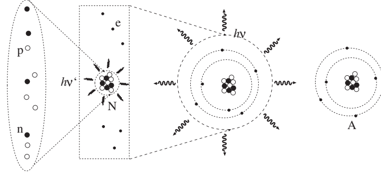
Figure 1: An atom (A) –self-contained structure– is obtained from a nucleus (N), previously assembled from protons (p) and neutrons (n), and an ensemble of electrons (e). Nucleus inertia \mathcal{M}_N = U_N c^{-2} decreases respect the inertia of its elementary particle components \mathcal{U}_N = 6m_p + 4m_n , due to the energy U_N - \mathcal{U}_N = -\tilde{U}_N = -8h\nu' released in its formation. Atom inertia \mathcal{M}_A = U_A c^{-2} decreases with respect to the inertia of its component nucleus and electrons \mathcal{U}_A = 6m_e + \mathcal{M}_N due to the energy U_A - \mathcal{U}_A = -\tilde{U}_A = -8h\nu released in its formation.
