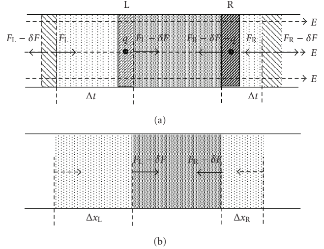
FIGURE 4: (a) A gas contained in a cylinder is compressed under the action of two pistons, L, with electric charge +q fixed to it, and R, with electric charge -q fixed to it. On piston L, a force F_L = qE is exerted by the electric field E and a force -(F_L - \Delta F) slightly smaller by the gas. On piston R a force F_R = -qE is exerted by the electric field, an a force (F_R - \Delta F) by the gas. (b) Thus the gas is compressed under the action of force F_L applied to a displacement \Delta x_L and a force F_R applied to a displacement \Delta x_R . Both forces F_L and F_R are applied simultaneously during time interval \Delta t . Every piston acts as an intermediate agent between the work reservoir (electric field and battery to which the capacitor is connected) and the thermodynamics system (the gas).
