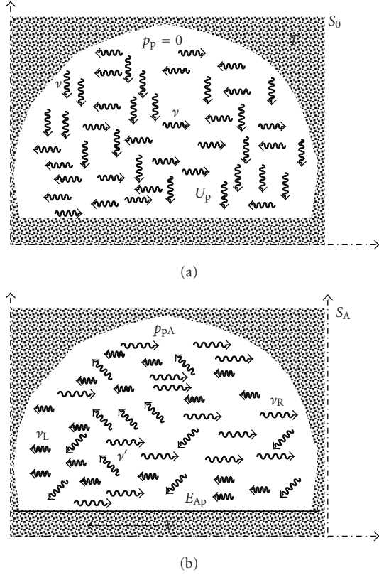
FIGURE 5: (a) Cavity with walls at temperature T filled with thermal radiation (photons) frequency \nu = \nu(T) (monochromatic approximation). In frame S_0 linear momentum for this ensemble of photons is zero p_p = 0 and its energy function is U_p = Nh\nu . (b) In frame S_A , the same ensemble of photons, with frequencies \nu_L > \nu , \nu_R < \nu (relativistic Doppler effect) and \nu' (aberration effect), has linear momentum p_{pA} = \gamma(V)(U_p c^{-1})V , according to the principle of inertia of energy, and total energy E_p = \gamma(V)U_p .
