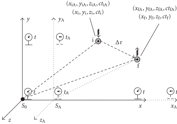
FIGURE 9: Frames S_0 and S_A in “standard configuration.” Axes y and z in both frames are parallel, and frame S_A moves with velocity V along axis x of frame S_0 . At time t = t_A = 0 origins coincide. Every frame has its own set of synchronized clocks. (i) Initial event, atom photon absorption, (f) final event, atom photon emission. \Delta\tau is the proper time of the atom (measured by a clock that travels with it) between events i and f.
