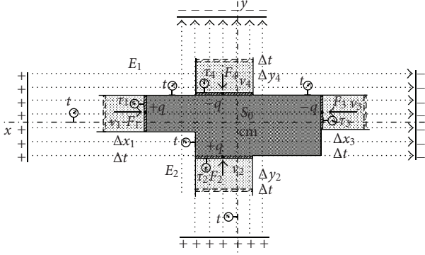
FIGURE 3: Extended system, with k pistons ( k = 1, 2, 3, 4 ), to which forces F_k = qE_k are simultaneously applied during time interval \Delta t as measured in frame S_0 by a set of synchronized clocks at rest (Figure 1). On the k th piston there is a clock that measures its proper time \tau_k . The k th piston displaces d\mathbf{r}_k during time interval dt , speed \mathbf{v}_k = d\mathbf{r}_k/dt , and proper time interval d\tau_k . Forces F_k have an electromagnetic origin: an electric field E_k , produced by a plane-parallel charged capacitor, interacts with a charge q_k fixed to the k th piston.
