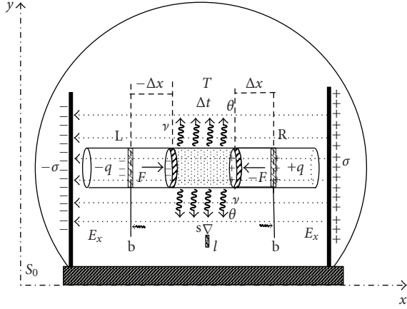
FIGURE 7: Cylinder with gas, diathermal walls, closed by two pistons, R and L, inside a plane-parallel capacitor with charge surface density \sigma . Laser (l), beam splitter (s), pistons of blocked mechanism (b) are used to assure that forces are applied simultaneously [62]. The gas in cylinder is compressed by forces acting on pistons. Force F_L = F acts on piston L during time interval \Delta t and displacement \Delta x_L = \Delta x . Force F_R = -F acts on piston R during time interval \Delta t and displacement \Delta x_R = -\Delta x . During the compression process, photons are emitted by cylinder walls with frequency \nu and zero linear momentum in frame S_0 .
